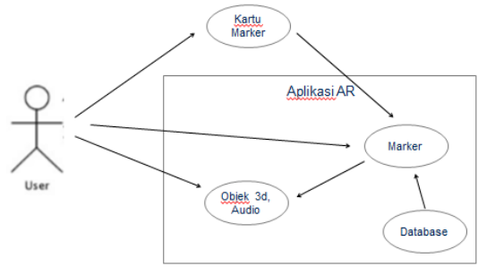
Gambar 3. Usecase diagram
