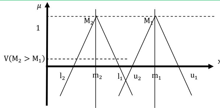
Figure 2. The intersection of M_1 and M_2
