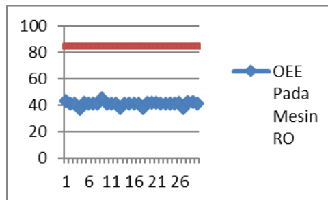
Gambar4.9 Grafik Pengukuran Overall Equipment Effectiveness Mesin RO mulai tanggal 1 sampai 30 november 2017
